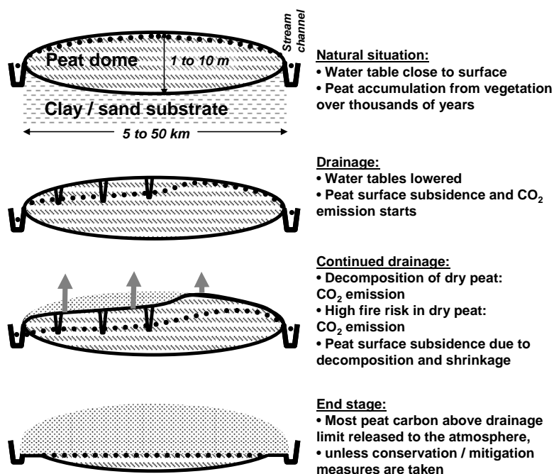
Fig. 1. Schematic illustration of CO 2 emission from drained peatlands.
