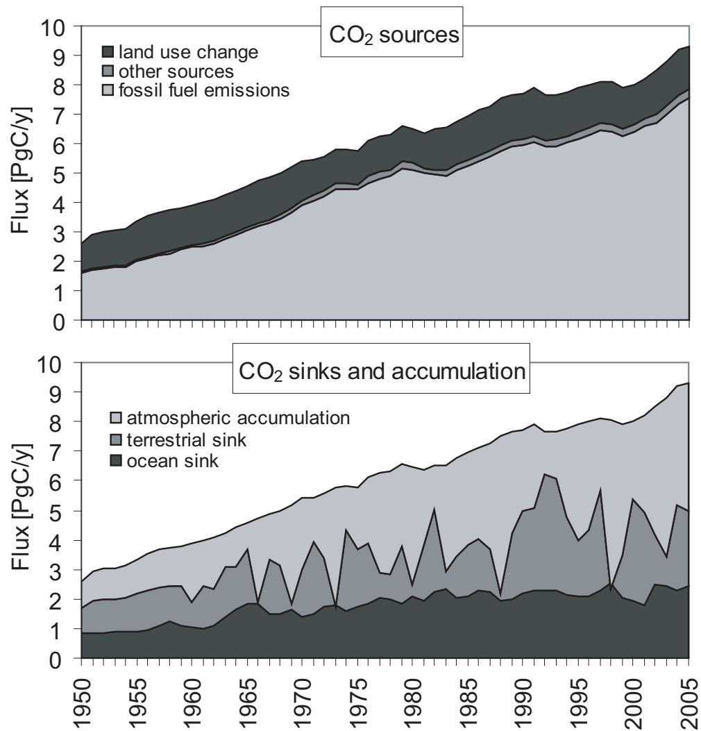
Figure 1: The global carbon budget for the period 1950-2005, showing terms in the CO 2 mass balance: [atmospheric CO 2 accumulation] = [emission flux from fossil fuels] + [other industrial emissions] + [emissions from land use change] - [flux to terrestrial sink] - [flux to ocean sink]. Data sources as in Canadell et al. 2007a, with atmospheric CO 2 change from ice core data (Law Dome, Antarctica; Etheridge et al. 1998b) before 1959 and direct measurements (Keeling and Whorf 2005) after 1959. Net terrestrial uptake is inferred by difference (total emissions less ocean uptake).
