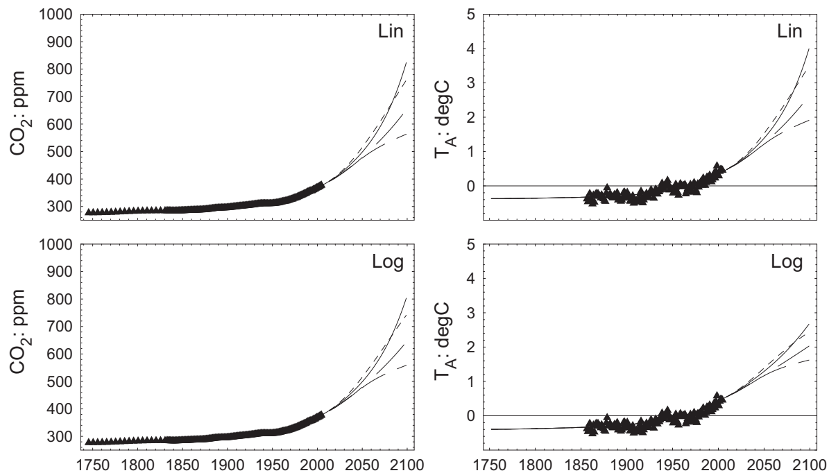
Figure 4: Predictions from a simple box model of the carbon-climate system of atmospheric \text{CO}_2 concentration ( [\text{CO}_2]_A , left panels) and global mean temperature ( T_A , right panels). The zero line for T_A is set to the average observed T_A over the period 1961 to 1990. Four emissions scenarios are shown, comprising actual fossil-fuel and land-use-change emissions from 1751 to 2005 (data sources as in Figure 1), and the A2 (solid), A1B (short dashed), B1 (medium dashed) and B2 (long dashed) scenarios (Nakicenovic et al. 2000) from 2005 to 2100. Upper and lower panels respectively show predictions with linear and logarithmic climate sensitivities to [\text{CO}_2]_A . Data (points) for [\text{CO}_2]_A are composite observations from ice core data from Law Dome, Antarctica (Etheridge et al. 1998b) (before 1959) and direct atmospheric measurements at Mauna Loa, Hawaii (Keeling and Whorf 2005) (1959 onward). Data (points) for T_A are the global temperature series 1850-2004 (Jones et al. 2006).
