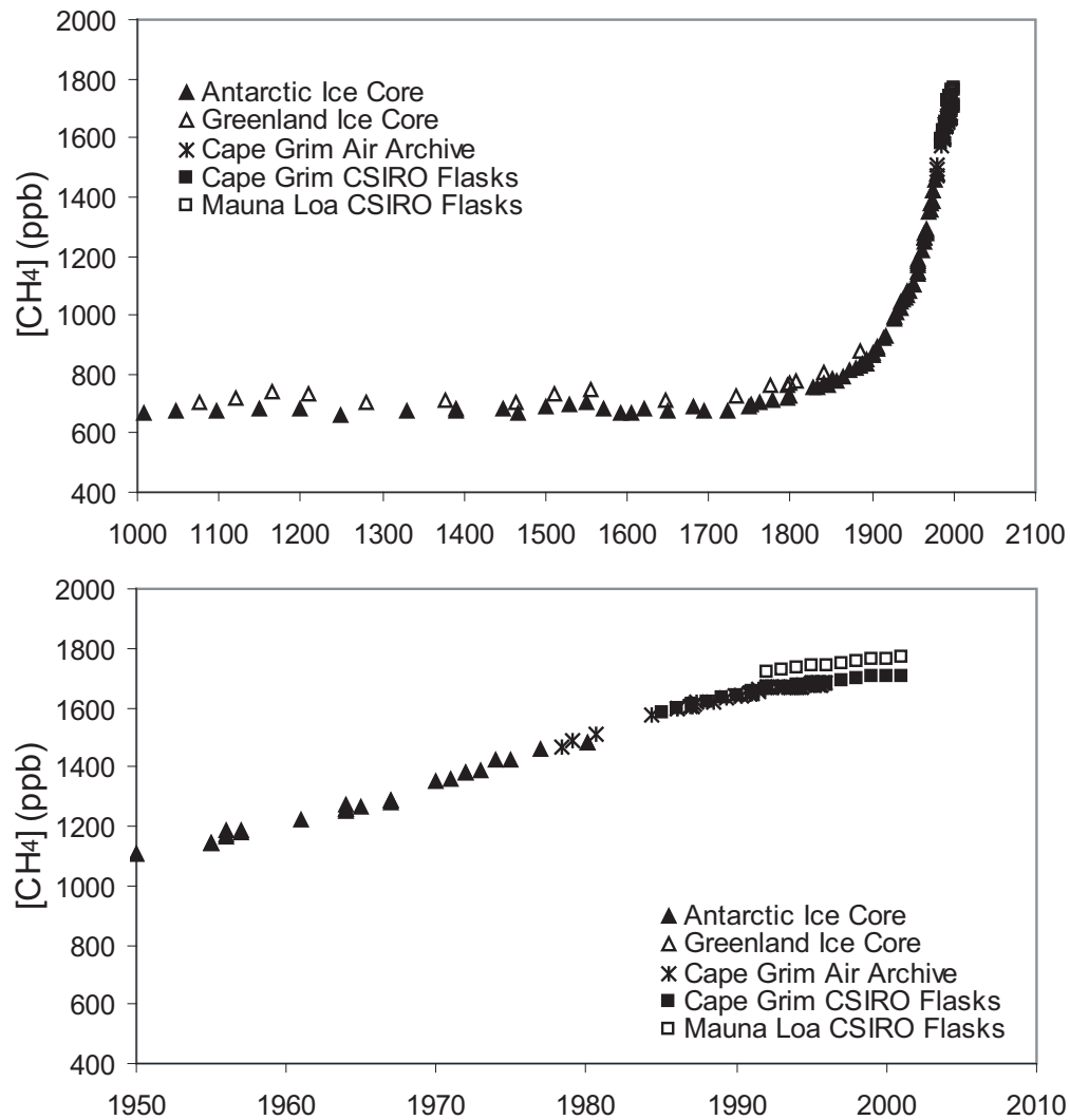
Figure 2: Atmospheric CH 4 concentrations from ice core data from Law Dome, Antarctica, and Summit, Greenland (Etheridge et al. 1998a); the Cape Grim Air archive (Etheridge et al. 1998a); and flask measurements at Cape Grim, Tasmania, and Mauna Loa, Hawaii (CSIRO flask network, archived at http://cdiac.ornl.gov/trends/atm_meth/csiro/csiro_gaslabch4.html ). Upper and lower panels show data on 1000-year and 50-year time axes, respectively.
