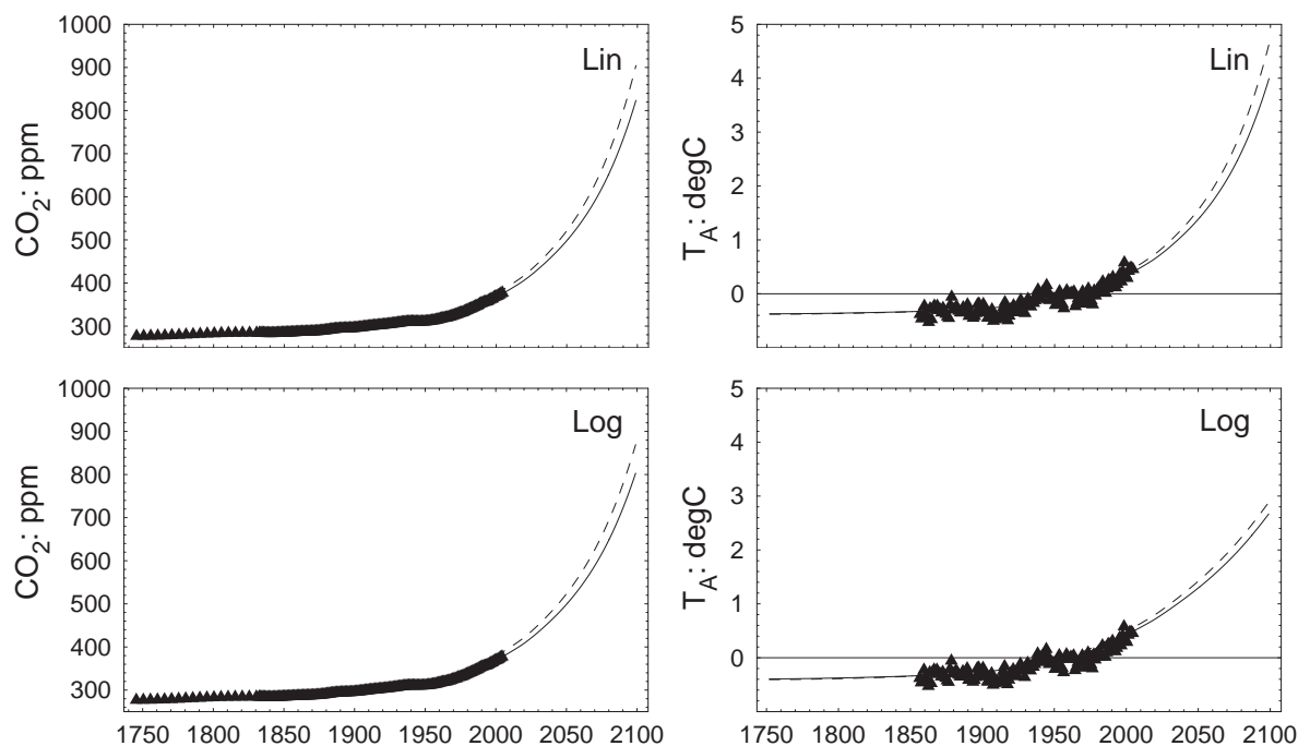
Figure 5: Predictions from a simple box model of the carbon-climate system of atmospheric \text{CO}_2 concentration ( [\text{CO}_2]_A , left panels) and global mean temperature ( T_A , right panels) without (solid) and with (dashed) feedbacks between the frozen carbon pool and global temperature. The emissions scenario comprises actual fossil-fuel and land-use-change emissions from 1751 to 2005 (data sources as in Figure 1), and the A2 scenario from 2005 to 2100. Upper and lower panels respectively show predictions with linear and logarithmic climate sensitivities to [\text{CO}_2]_A . Data for [\text{CO}_2]_A and T_A as in Figure 4.
