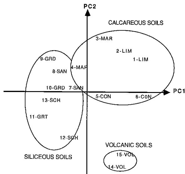
Fig. 1. Principal component analysis of the soil data for the fifteen soils derived from eight parent materials. Abbreviations: LIM-limestone, MAR-marl, CON-conglomerate, SAN-sandstone, GRD-granodiorite, GRT-granite, SCH-schiste, VOL-volcanic rock. The corresponding stand numbers are shown in Table 1.
