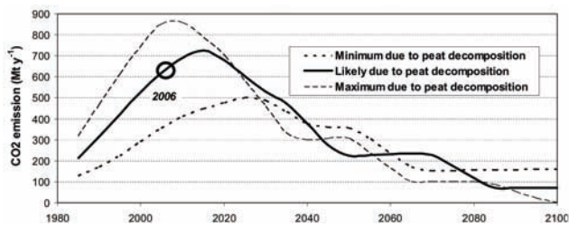
Fig. 5. Historical, current and projected CO 2 emissions from peatlands, as a result of drainage (fires excluded). The increase in emissions is caused by progressive drainage of an increased peatland area. The following decrease is caused by peat deposits being depleted, starting with the shallowest peat deposits that represent the largest peatland area. The stepwise pattern of this decrease is explained by the discrete peat thickness data available (0.75 m, 1.5 m, 3 m, 6 m, 10 m). The “minimum”, “likely” and “maximum” lines correspond with possible drainage intensities as presented in Table 1.
