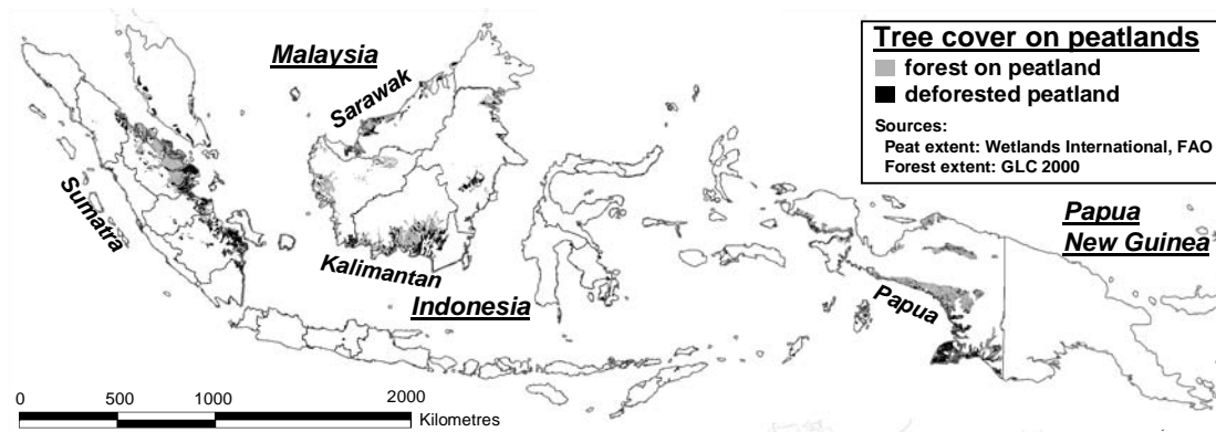
Fig. 2. Forest cover on peatland in the year 2000 (GLC 2000 land cover data; Bartholomé and Belward 2000), in Indonesia, Malaysia and Brunei.
