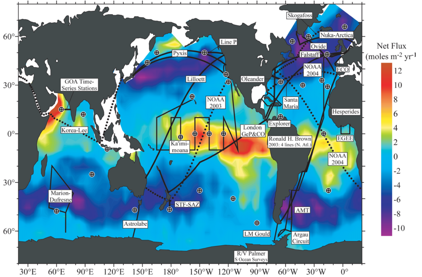
Fig. 2. In this global map of existing and planned near-surface pCO_2 measurements, solid lines indicate existing lines. Dashed lines indicate planned lines that are not operational at this time. Labels indicate ship name or project title. White circles with crosses indicate preliminary estimates of planned and existing time-series stations with surface CO_2 measurements. The background map shows net annual CO_2 flux adapted from Takahashi et al., [2002].
